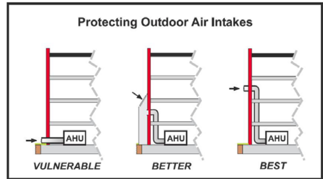
Figure 3. Outdoor HVAC air intakes (NIOSH).
